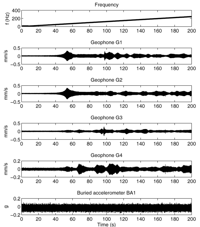
FIG. 7—Response of geophones and buried accelerometer in test C003 (small v_0 ).
